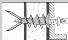
3. SCREW & TIGHTEN
